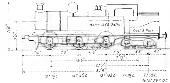
Fig. 1—Type of Locomotive That Was Used in Making Spring Tests
